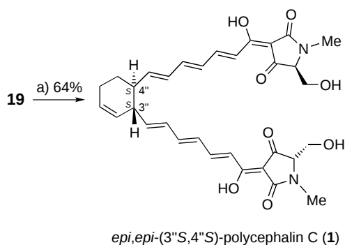
Scheme 8. Synthesis of epi, epi -(3'' S ,4'' S )-polyccephalin C ( 1 ). a) TFA/H 2 O (9:1) \times 3, RT (64 %).
