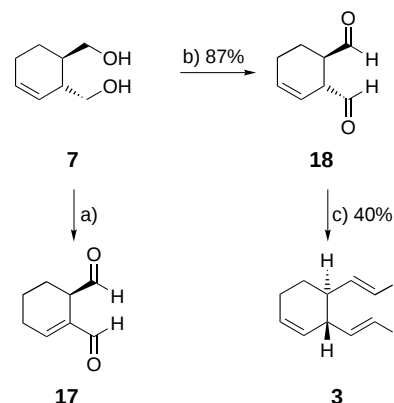
Scheme 6. Synthesis of bis-iodovinyl fragment 3 . a) (\text{COCl})_2 , \text{DMSO} , \text{CH}_2\text{Cl}_2 , -78^\circ\text{C} , 2 h; then \text{NEt}_3 , -78 \rightarrow -10^\circ\text{C} ; b) (\text{COCl})_2 , \text{DMSO} , \text{CH}_2\text{Cl}_2 , -78^\circ\text{C} , 1.5 h; then i\text{Pr}_2\text{NEt} , -78 \rightarrow -10^\circ\text{C} ; c) \text{CrCl}_2 , \text{CHI}_3 , \text{THF} , 0^\circ\text{C} \rightarrow \text{RT} , 2 h.
