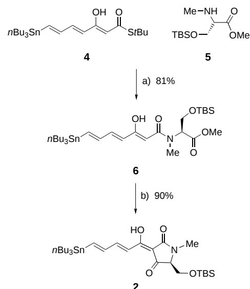
Scheme 2. Synthesis of dienoyltetramic acid 2 . a) CF 3 CO 2 Ag, NEt 3 , THF, 0 °C, 20 min; b) NaOMe, MeOH, 25 °C, 2 min.
